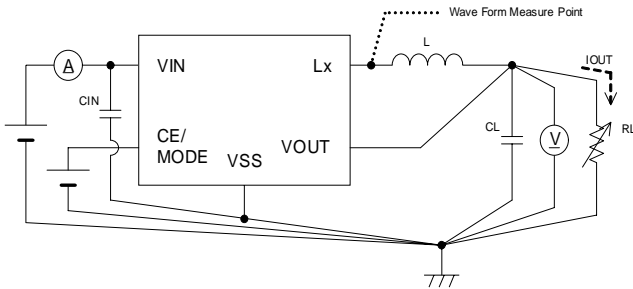
Circuit ①
