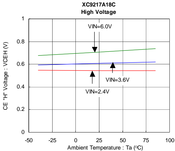
(8) CE "H" "L" Voltage vs. Ambient Temperature
